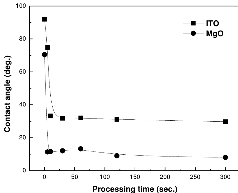
Fig. 2. Effect of plasma exposure time on the contact angles of ITO and MgO surfaces after the cleaning by a perforated dielectric covered DBD with N_2 (200 sccm)/(4500 sccm He + 45 sccm O_2 ) at 5 kV of AC voltage.
