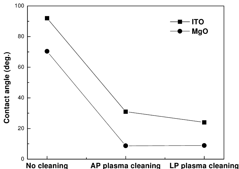
Fig. 3. Contact angles of ITO and MgO surfaces after the cleaning for 2 min by a low-pressure oxygen plasma using an inductively coupled plasma equipment with 200 W of inductive power at 13 Pa. As references, the contact angles of as-received, and atmospheric pressure plasma cleaned ITO and MgO surfaces (for 2 min) shown in Fig. 2 are also shown.
