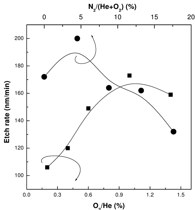
Fig. 1. Effect of various gas combinations such as He/ O_2 and N_2 /(He+ O_2 ) on the photoresist etch rate. AC voltage was maintained at 6 kV and He at 4500 sccm. O_2 was varied from 9 to 63 sccm and N_2 from 0 to 800 sccm.
