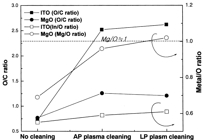
Fig. 4. The ratios of O/C and metal/O on the ITO and MgO surfaces measured by XPS after the cleanings by the atmospheric pressure plasma and by the low-pressure ICP shown in Fig. 3. As a reference, the ratios of O/C of as-received ITO and MgO surfaces were included in the figure.
